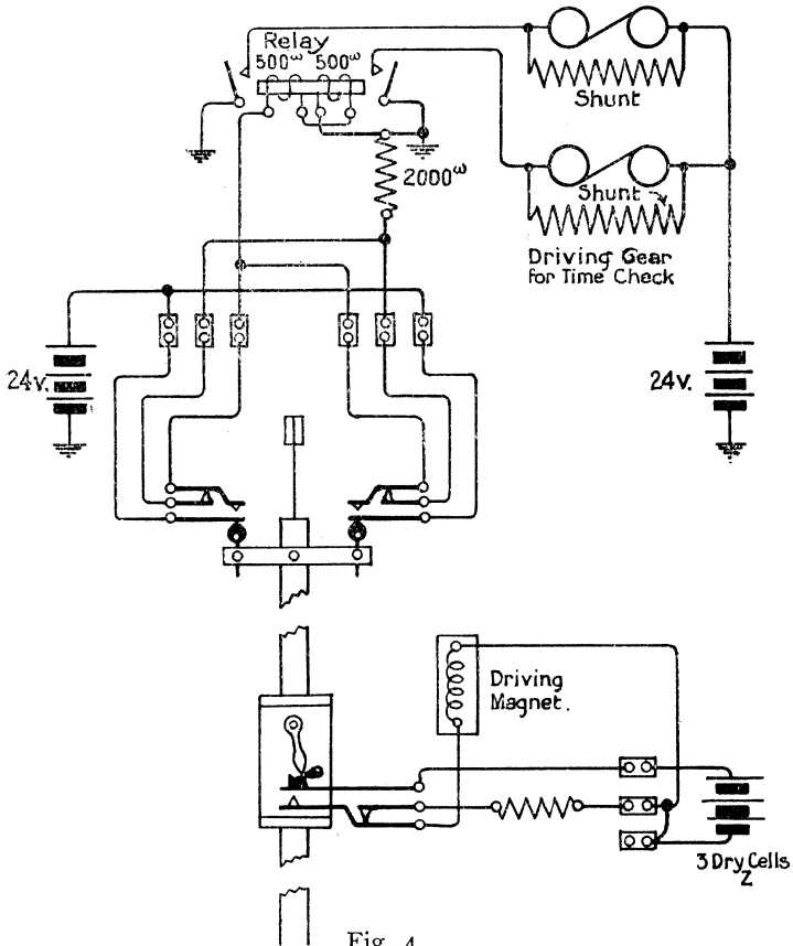
Fig. 4. PENDULUM ELECTRICAL SECONDS (Bowel), FOR DRIVING TIME CHECKS.
