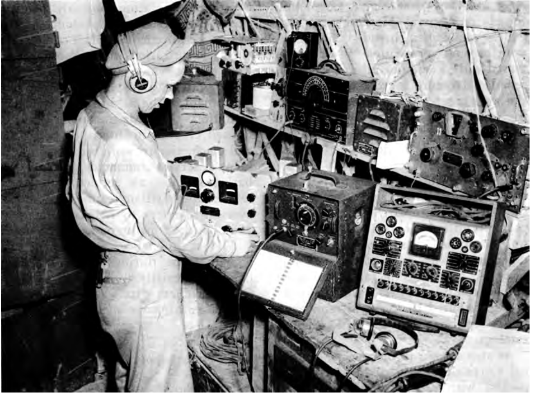
CHECKING THE FREQUENCY OF A BC-779-A RECEIVER at the signal repair section of General Stilwell's headquarters, Burma.
