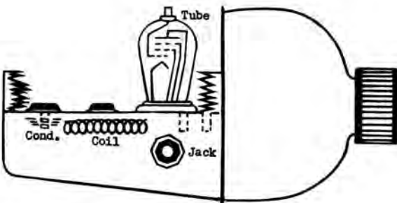
DRAWINGS OF A CANTEEN RADIO
