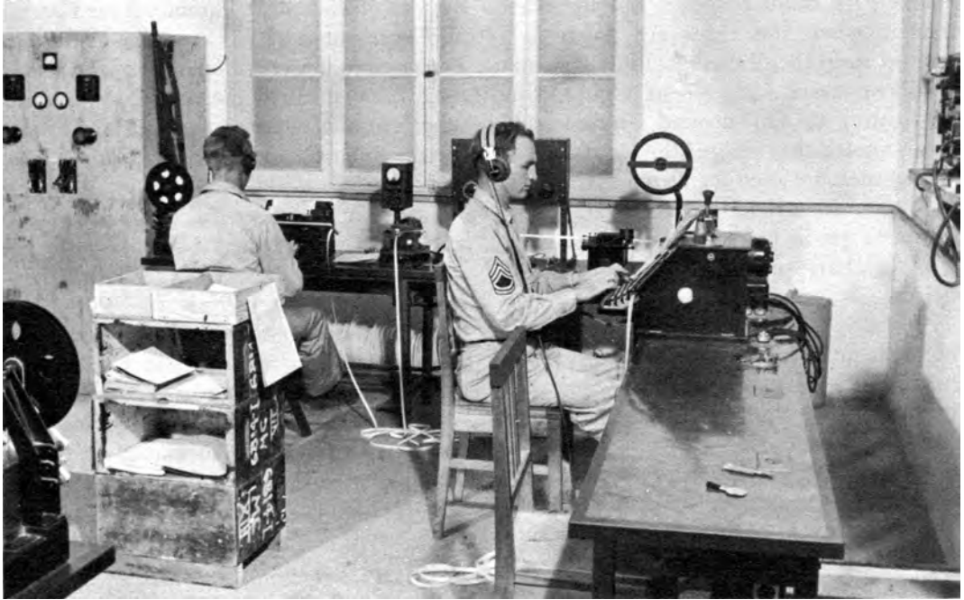
BOEHME HIGH-SPEED OPERATION in the base message center at Nouméa.
