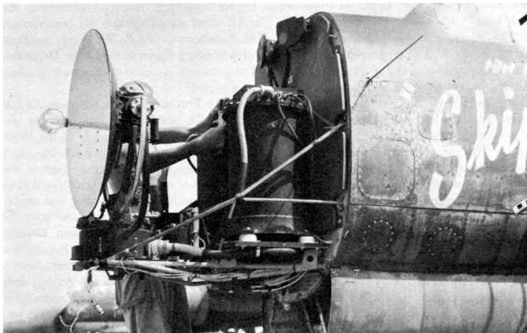
AIRBORNE AI-10 RADAR, SCR-520
