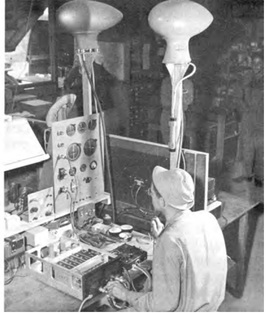
INSTALLATION AND MAINTENANCE OF SIGNAL EQUIPMENT included such assignments as installing radio equipment in aircraft (left, above), repairing radio compasses (right, above) in Australia, and the operation of general repair shops (below) in New Guinea.
