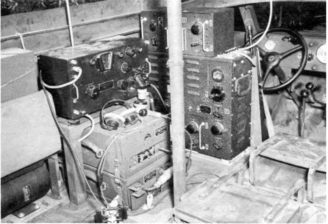
VEHICULAR MOUNTING OF RADIO SETS. The SCR-510 and SCR-193.
