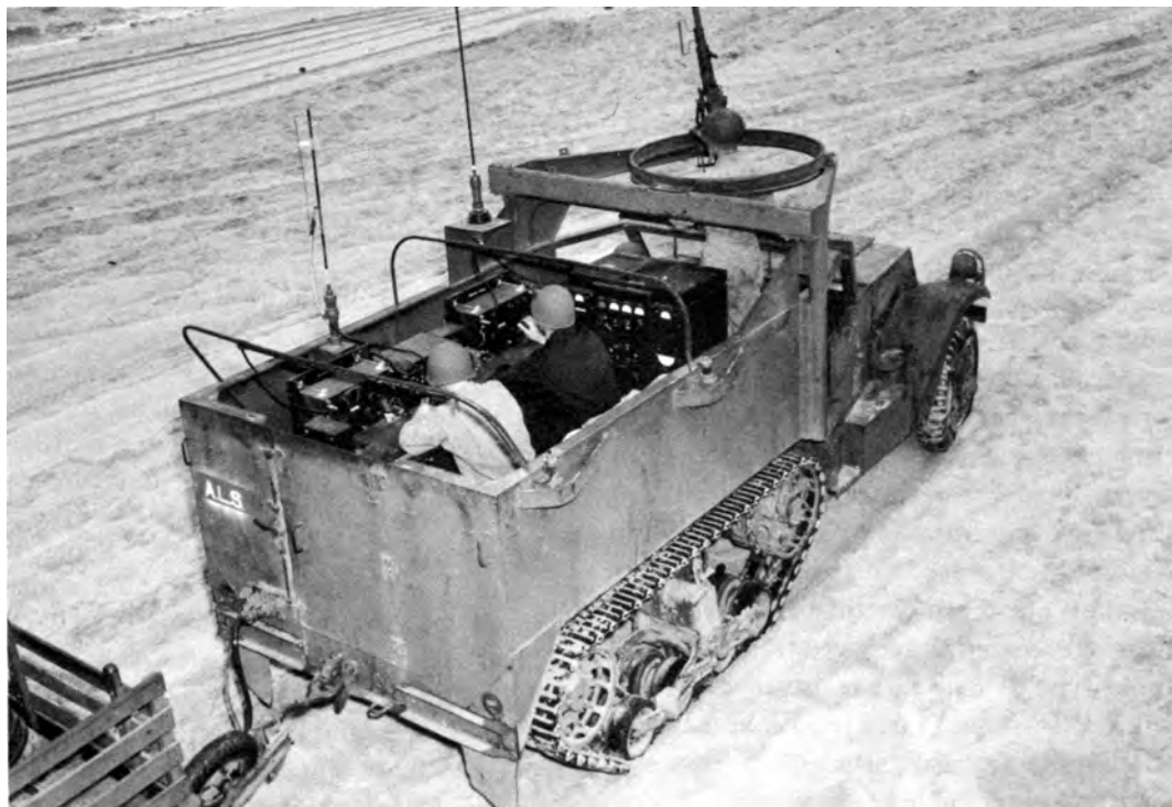
VEHICULAR MOUNTING OF RADIO SETS. The SCR-299.
